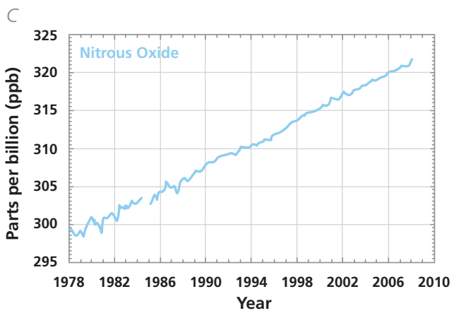
Figure 5 The trends in atmospheric concentrations for the greenhouse gases (A) carbon dioxide, CO 2 , in ppm (parts per million) from 1958 to present 13 ; (B) methane, CH 4 , in ppb (parts per billion) from 1979 to present 14 ; and (C) nitrous oxide, N 2 O, in ppb (parts per billion) from 1978 to present 2,13,14,15 .
